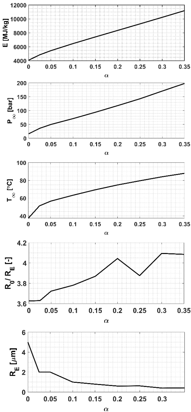
Fig. 5 The variation of the optimal control parameters as a function of the accommodation coefficient
