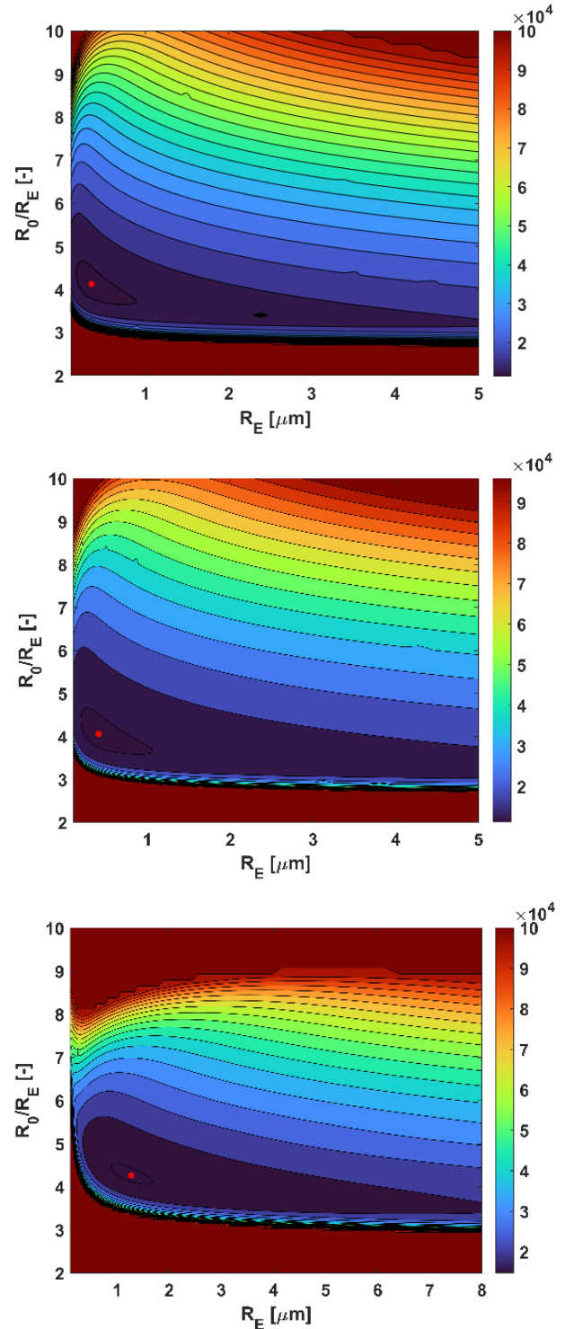
Fig. 3 Bi-parametric maps at different ambient properties. Top to down: 20 bar and 60 °C; 198 bar and 87 °C (optimal); and 300 bar and 96 °C.
