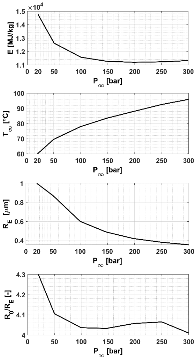
Fig. 4 Optimal energy intensity values and parameter combinations as a function of the ambient pressure
