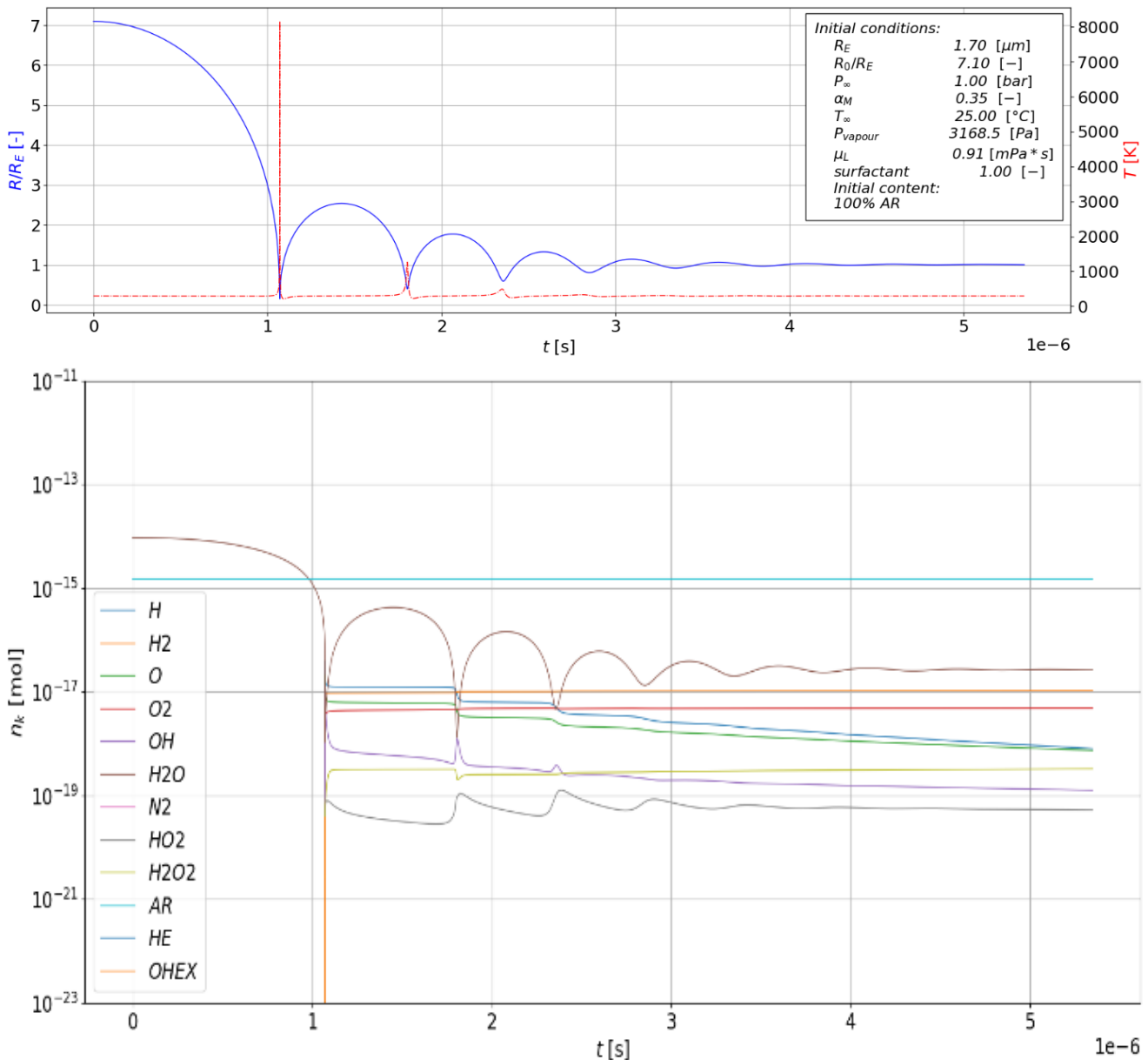
Fig. 1 A typical example of the dynamics of a freely oscillating microbubble. Top panel: bubble radius (blue) and internal temperature (red) as a function of time. Bottom panel: temporal evolution of the chemical species in moles.
