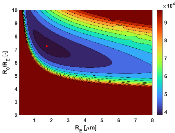
Fig. 2 Energy intensity of hydrogen production (in terms of MJ/kg) at 1 bar and 25 °C as a function of the bubble radius and expansion ratio. The dot represents the optimum parameter combination.
