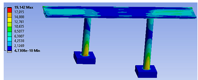
Fig. 4 Stress distribution in the bridge lateral loading
