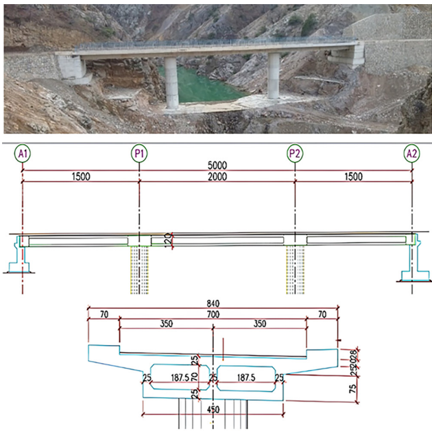
Fig. 1 Artvin Ardanuc Incesu Bridge
