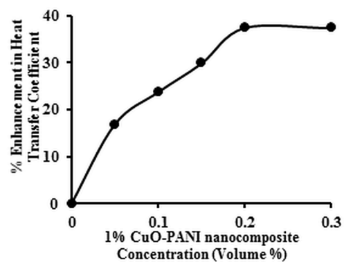
Fig. 10 Effect of 1% CuO–PANI nanocomposite concentration in nanofluid on heat transfer coefficient enhancement (at x/D_i = 761.5 i.e. at outlet of the helical coil and Re = 1890 \pm 5 )
