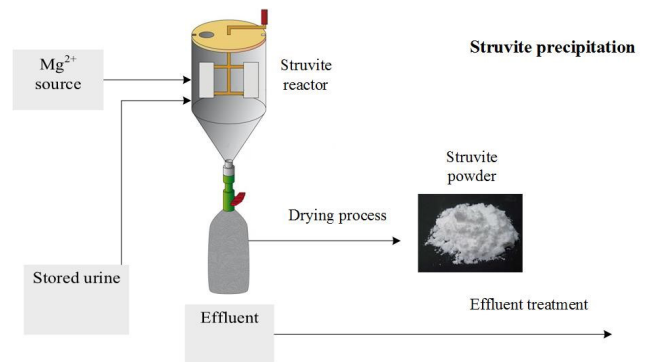
Fig. 4 Production of struvite by chemical addition (modified sketch based on [44])
